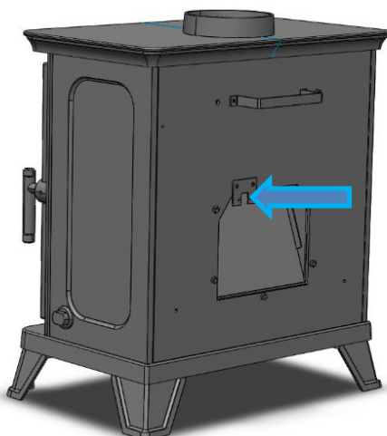
Fig.3 Thermal switch bracket
