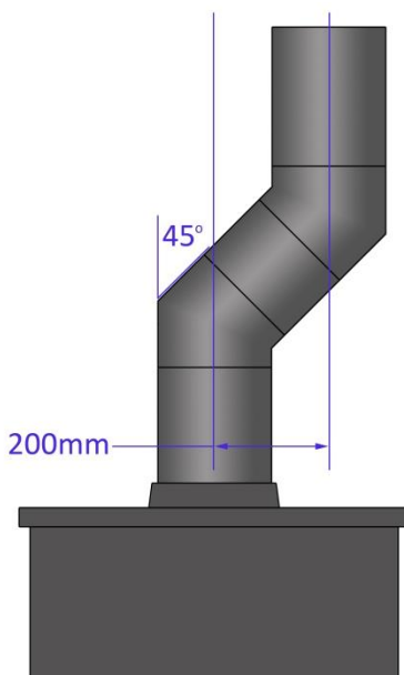
Fig.6 Flue offset
