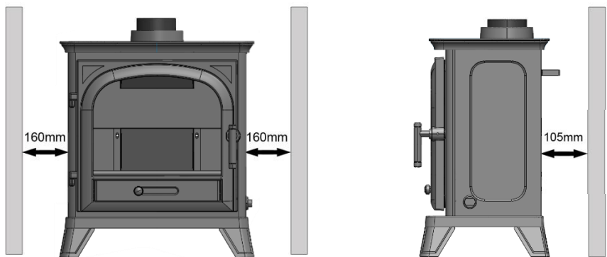
Fig.5 Clearances
