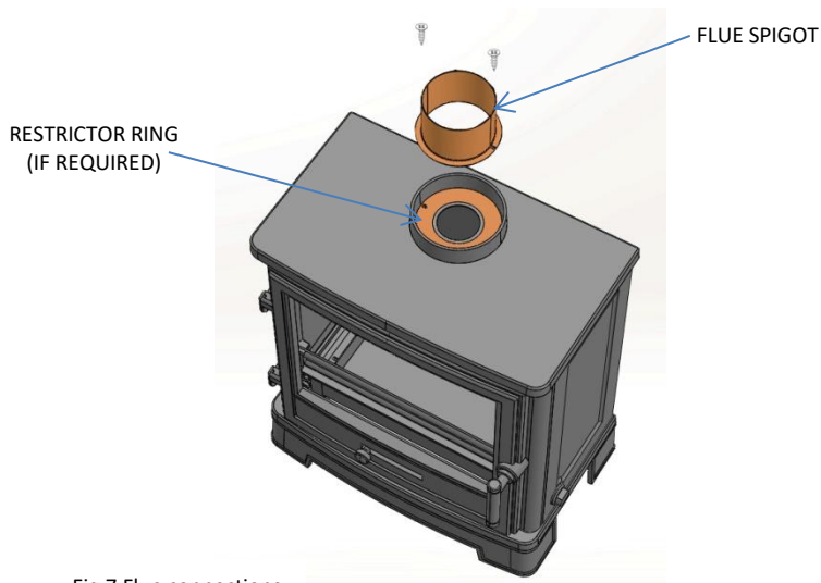
Fig.7 Flue connections
