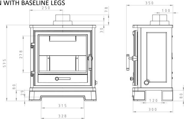
GAS BASSINGTON WITH BASELINE LEGS
