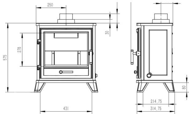
GAS BASSINGTON WITH SKIRTED LEGS
