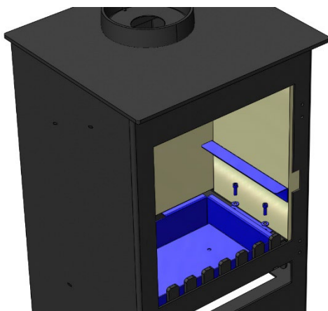
Fig.3 Burner Tray Fitting
