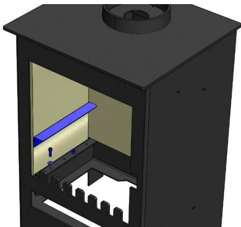
Fig.2 Mesh Trims
